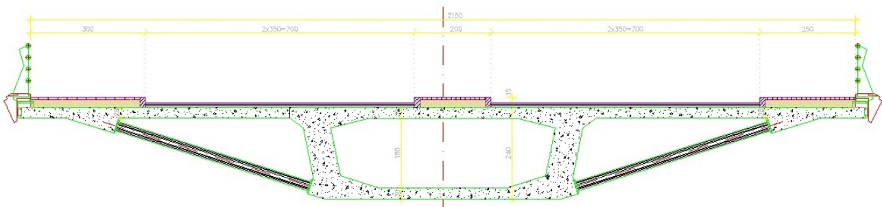
Final cross-section of main girder
