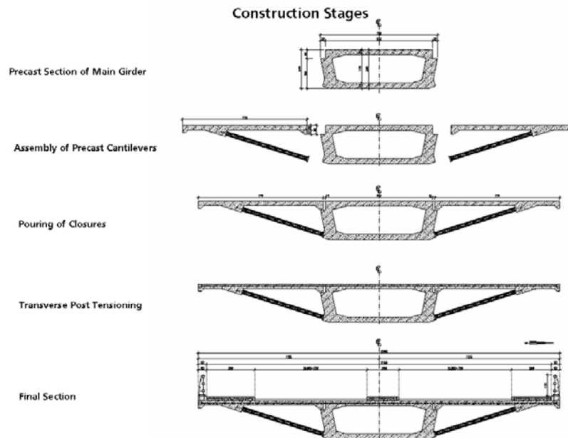
Staged construction of cross-section.
