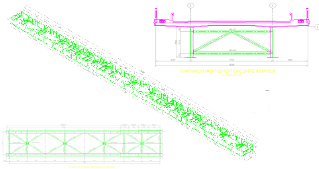
Representation of steel components and typical cross-section
