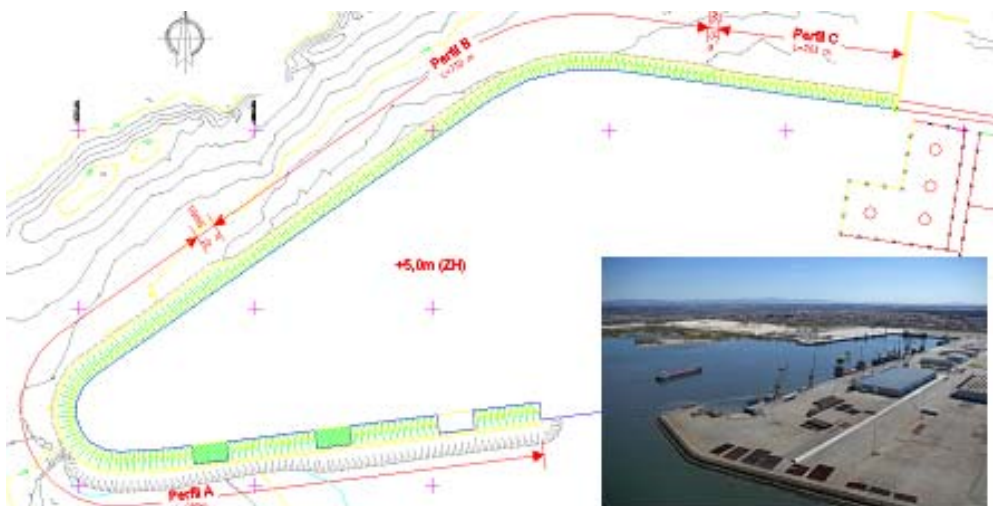
Plan view and photograph of the new port of Aveiro.
