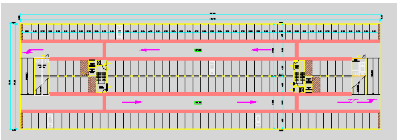
Floorplan
