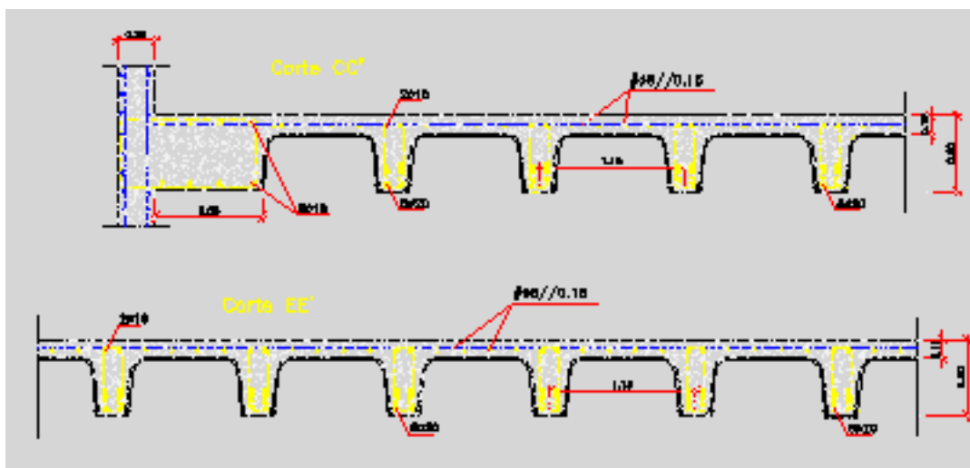
Cuts
