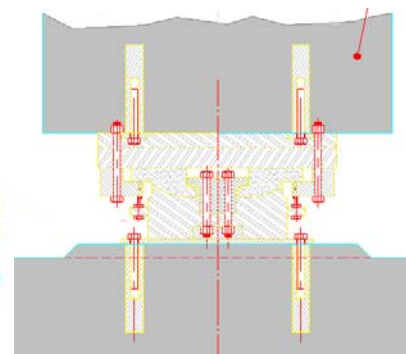
Bearing detail
