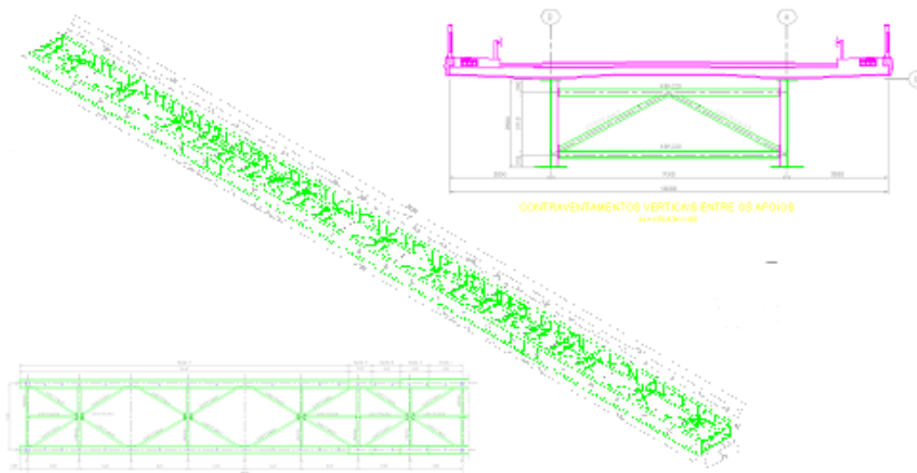
Representation of steel components and typical cross-section
